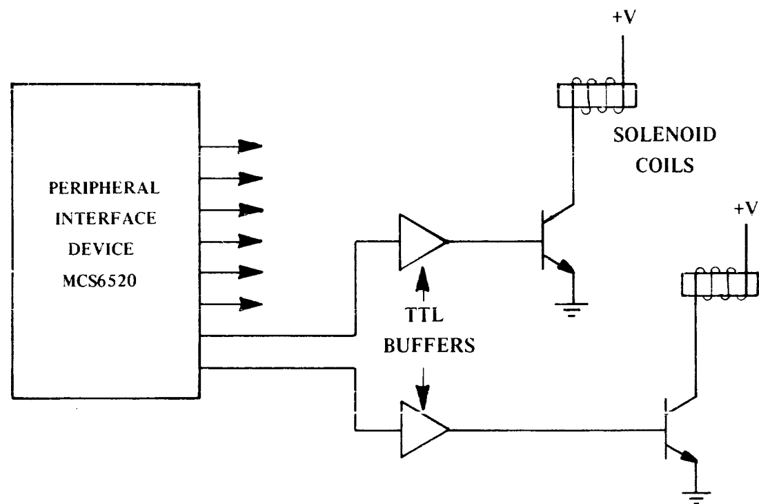
MCS6520 Driving TTL Buffers FIGURE 2.4
